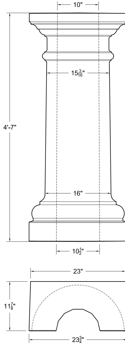
CT 4'-7x16 Half-Col ± 355 LBS
