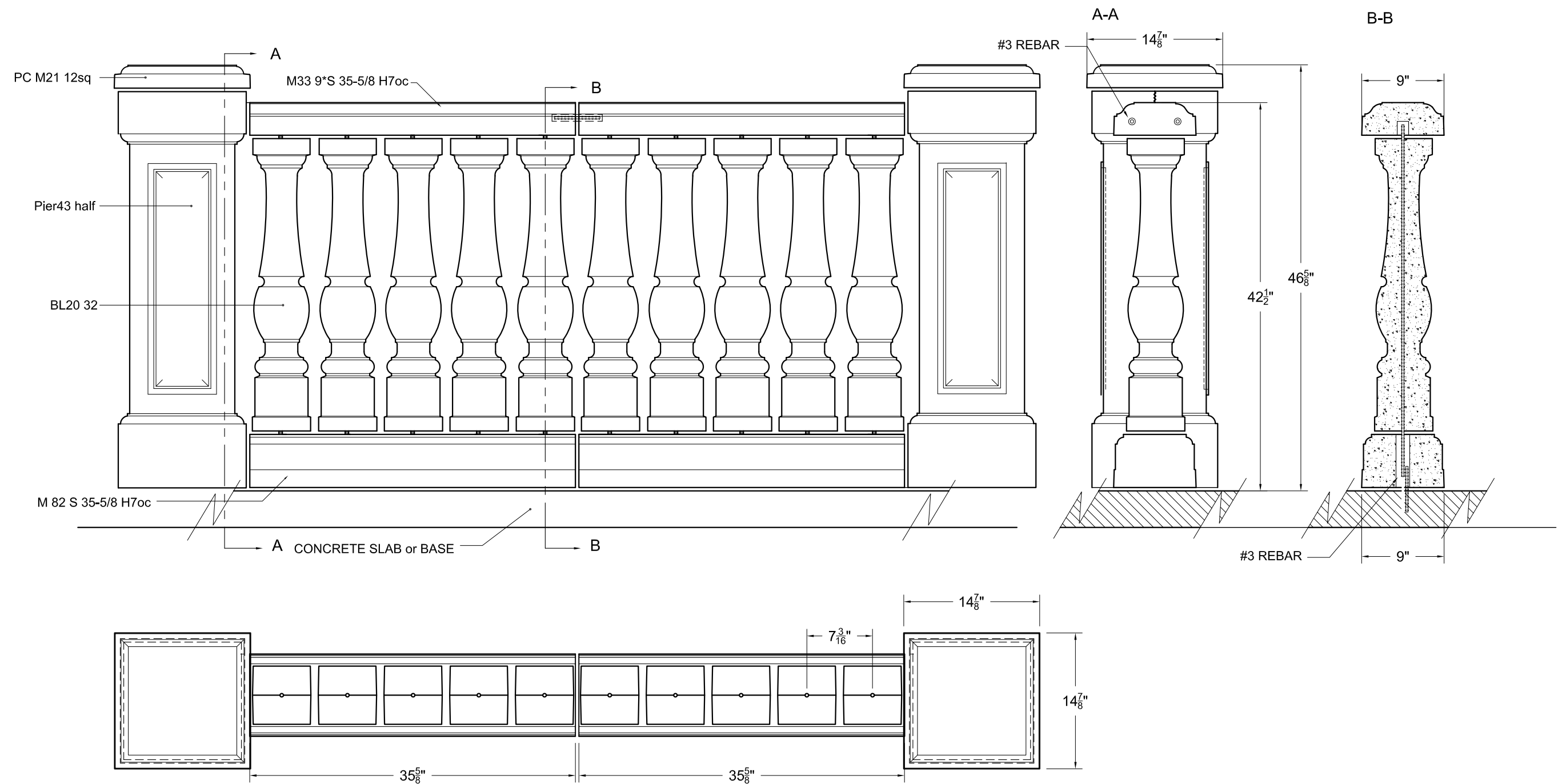
1 PIER 43 & BL20-32 Balustrade Assembly, 7in o.c., Typical
